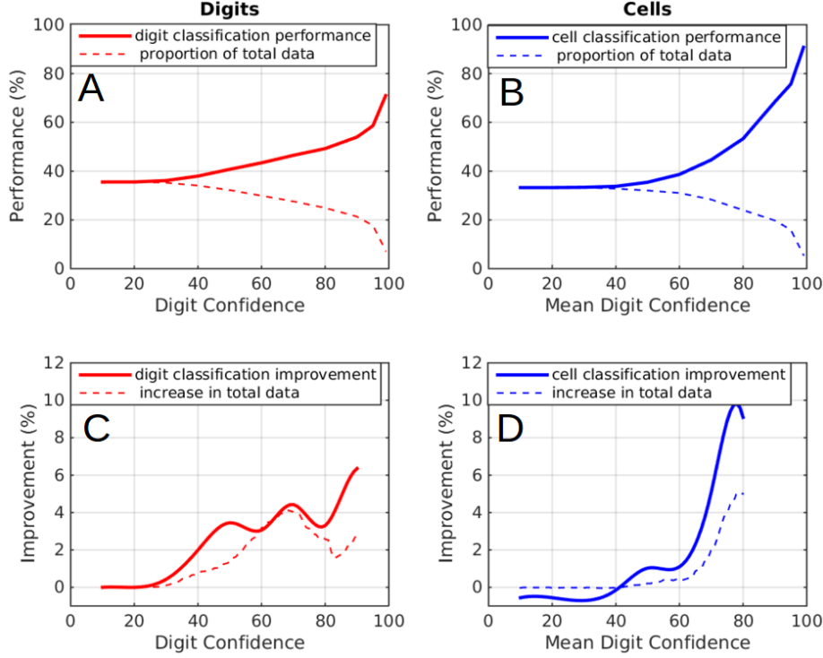
Figure 4. The accuracy of the Multiclass Support Vector Machine in digit and cell level classification and the improvement in accuracy on a held-out test set after retraining the algorithm with 50% of the collected data. (A) shows the digit level classification, (B) shows cell level classification, (C) shows improvements in digit classification after feedback of human annotations (D) shows improvements in cell classification after feedback of human annotations. The "mean digit confidence" refers to the mean confidence of the MSVM across all individual digits within the cell.
